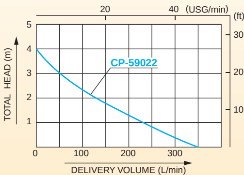
Performance Curve
