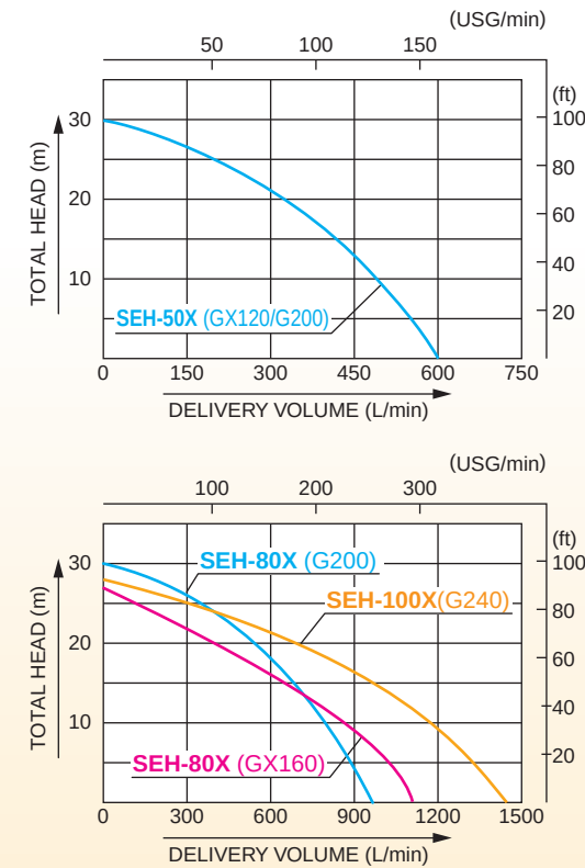
■ Performance Curve
